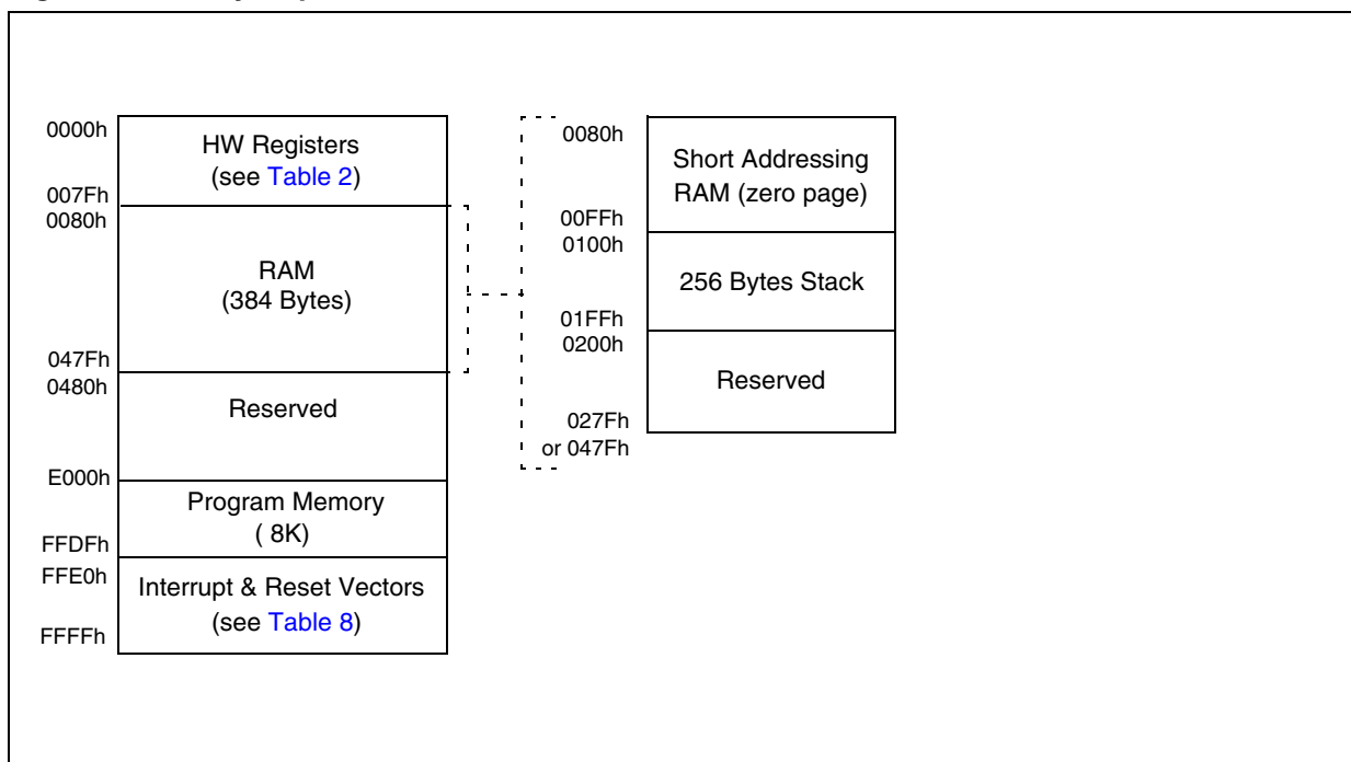
Figure 4. Memory Map
