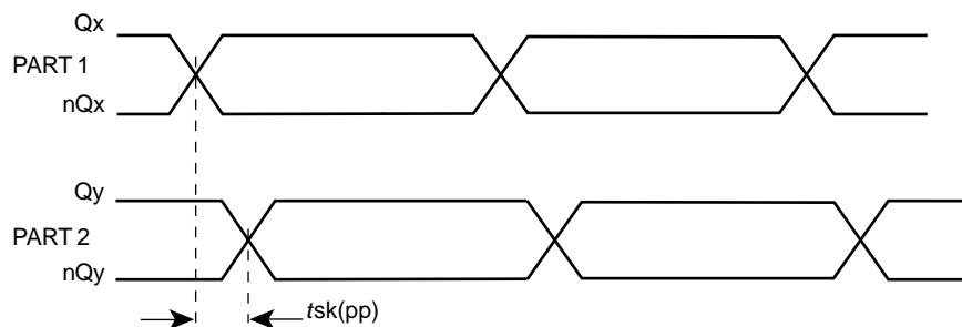
FIGURE 2 - PART-TO-PART SKEW
