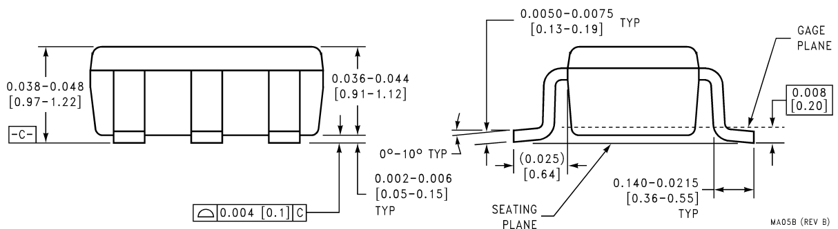
SOT23-5 Package NS Package Number MA05B
