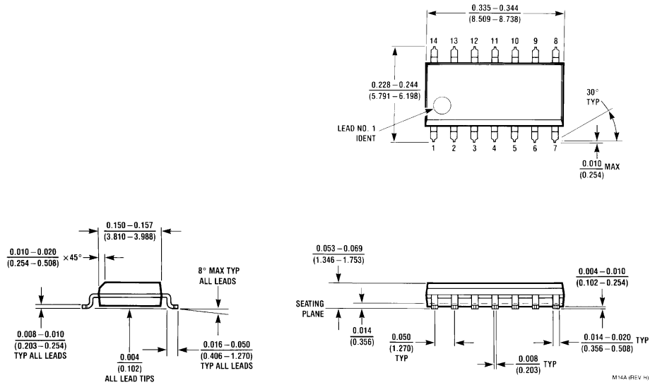
14-Pin Small Outline Package Order Number LM6144AIM or LM6144BIM NS Package Number M14A
