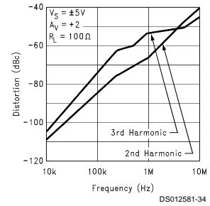
Harmonic Distortion vs Frequency ( V_S = \pm 5\text{V} )
