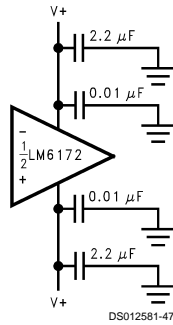
FIGURE 5. Power Supply Bypassing
