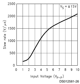
Slew Rate vs Input Voltage
