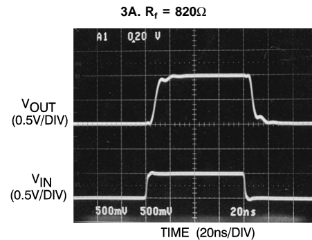
FIGURE 3. Increase Compensation by Increasing R_f , A_V = +2
