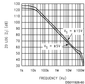
Transimpedance vs Frequency R_L = 1 k\Omega
