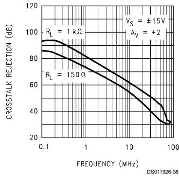
FIGURE 12. Crosstalk Rejection
