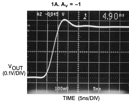
FIGURE 1. Variation of Closed-Loop Gain from -1 to -5 Yields Similar Responses.
