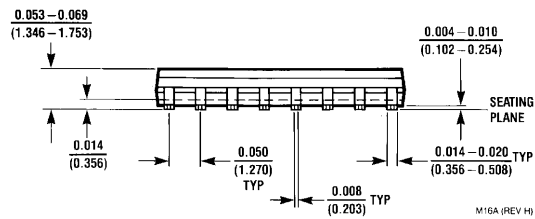
Small Outline Package (M) Order Number LM6182IM or LM6182AIM NS Package Number M16A
