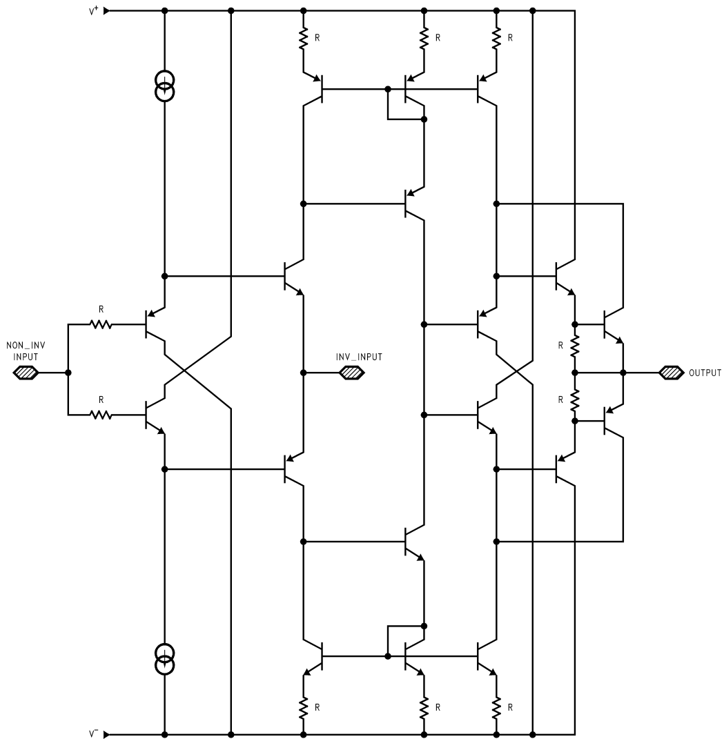
Simplified Schematic 1/2 LM6182
