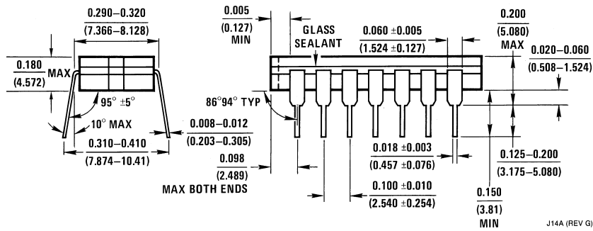
14-Lead Dual-In-Line Package (J) Order Number LM6182AMJ/883 NS Package Number J14A
