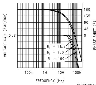
Inverting Gain Frequency Response V_S = \pm 5V, A_V = -1, R_f = 820\Omega
