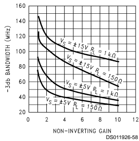
Non-Inverting Gain vs -3 dB Bandwidth R_f = 820\Omega
