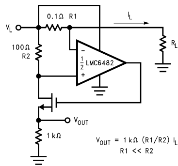
FIGURE 22. Positive Supply Current Sense
