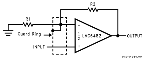
Non-Inverting Amplifier
