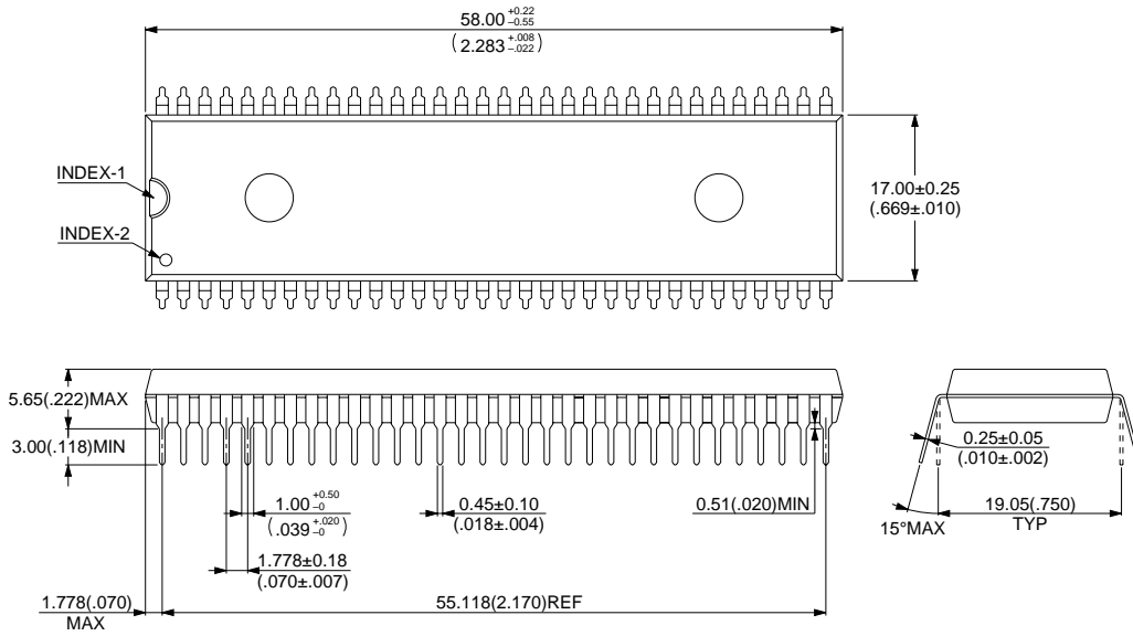
64-pin Plastic SH-DIP (DIP-64P-M01)
