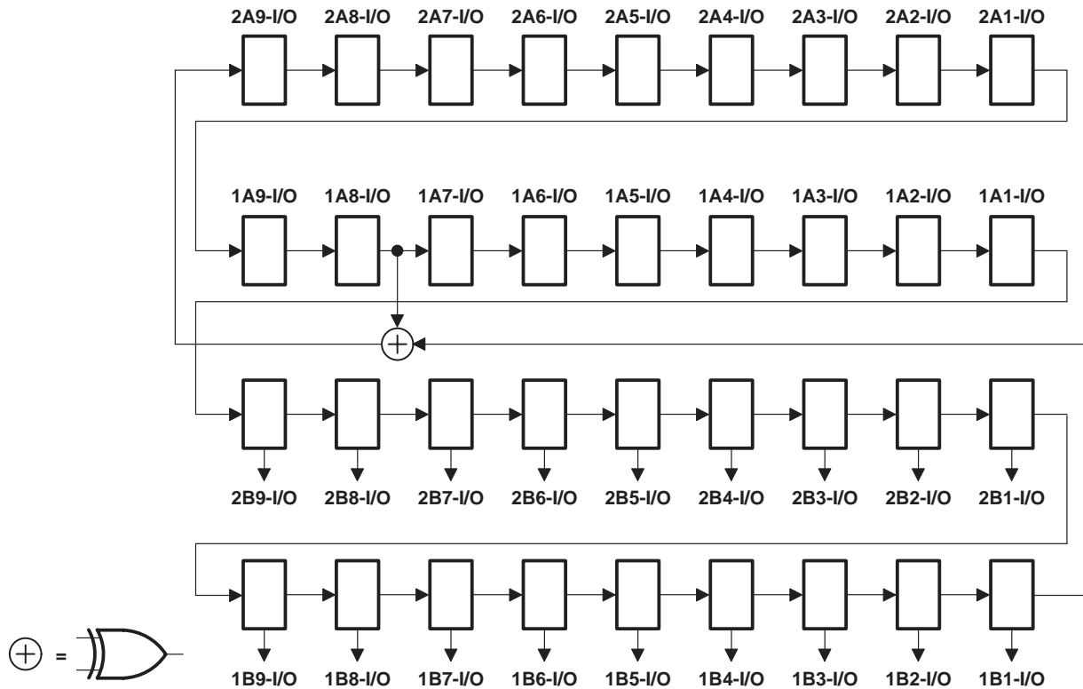
Figure 6. 36-Bit PRPG Configuration ( 1OEAB = 2OEAB = 1 , 1\overline{OEBA} = 2\overline{OEBA} = 1 )
