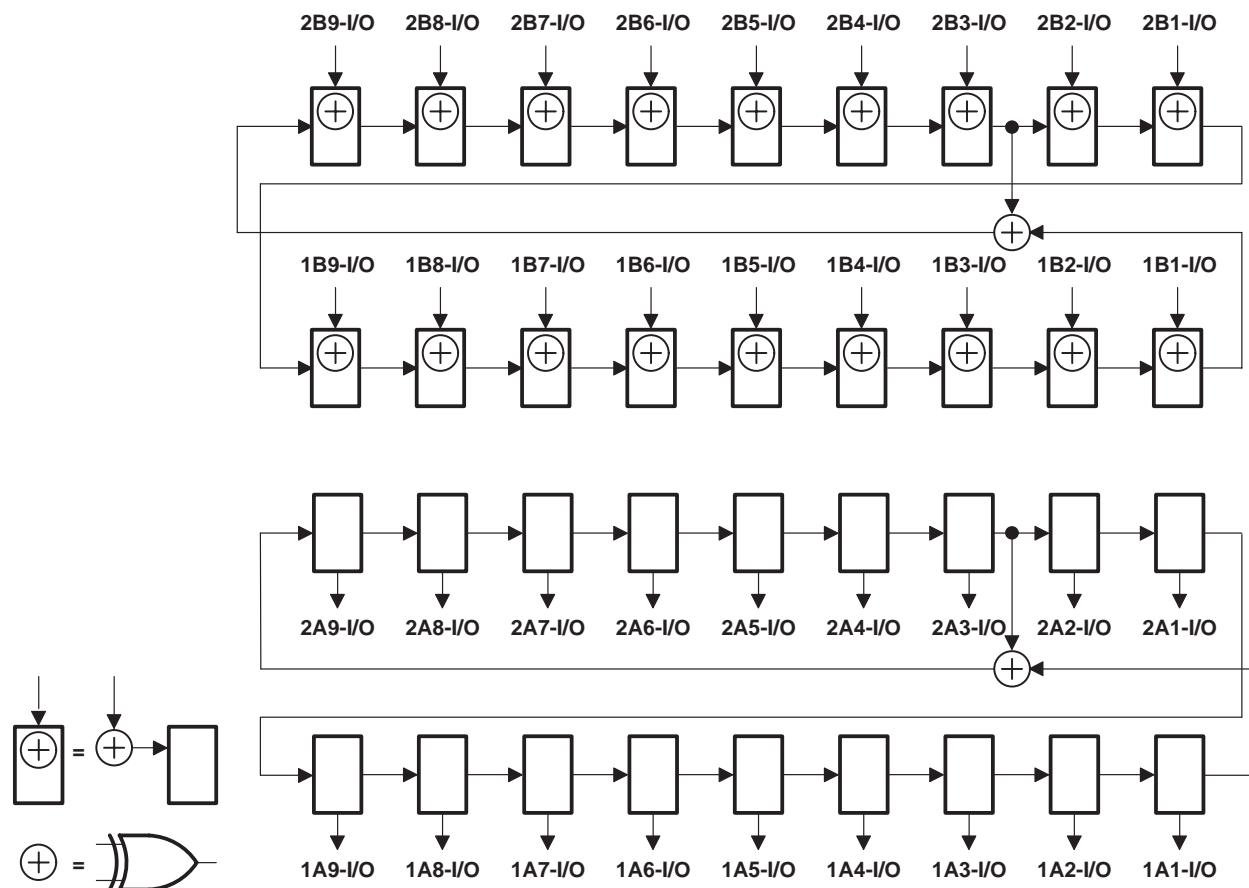
Figure 11. 18-Bit PSA/PRPG Configuration ( 1OEAB = 2OEAB = 0 , 1\overline{OEBA} = 2\overline{OEBA} = 0 )
