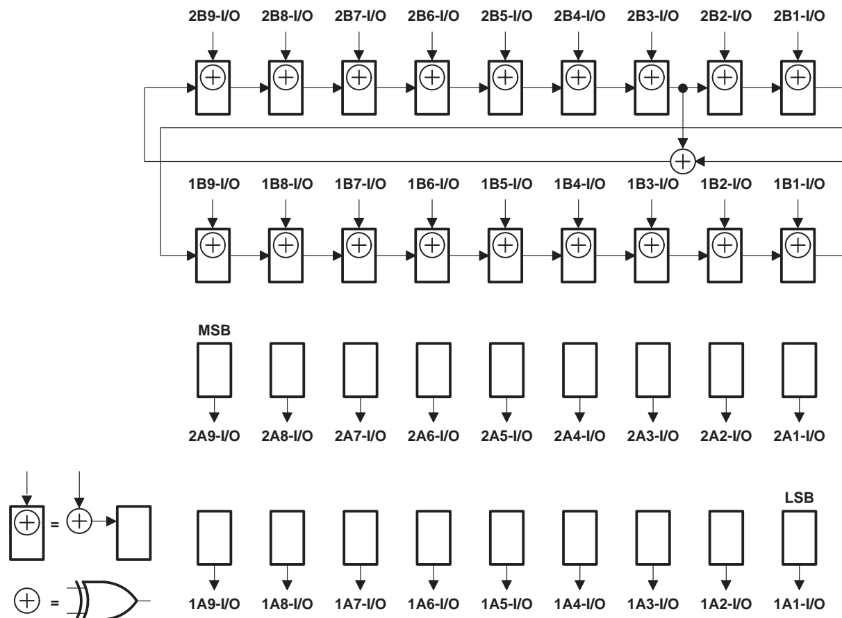
Figure 13. 18-Bit PSA/COUNT Configuration ( 1OEAB = 2OEAB = 0 , 1\overline{OEBA} = 2\overline{OEBA} = 0 )
