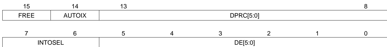
Figure 3-22. DMPREC Register
