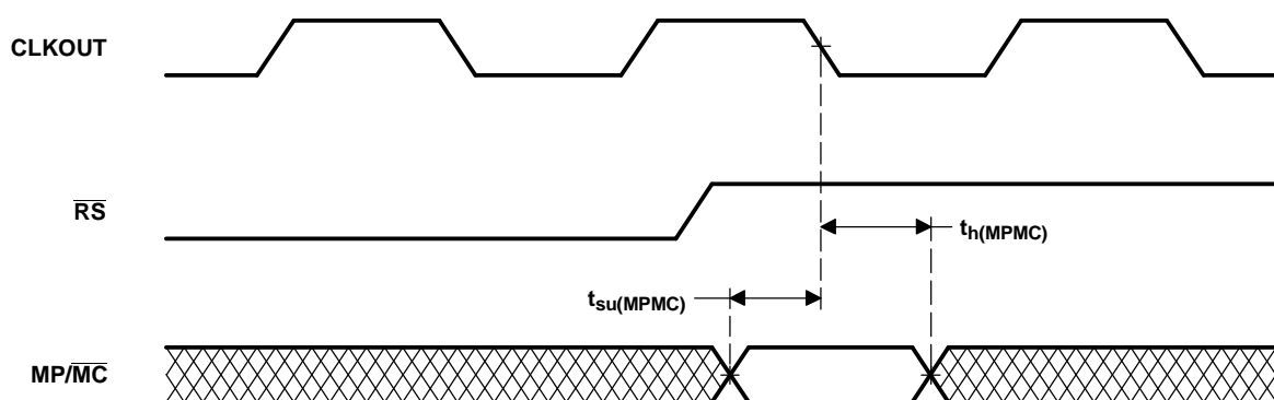
Figure 5-17. MP/MC Timing
