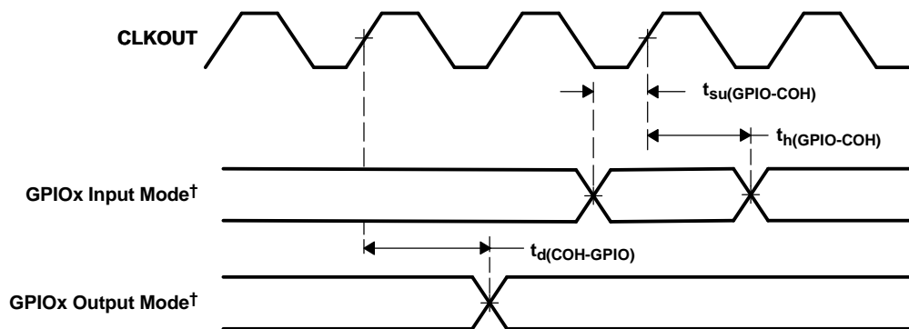
Figure 5-31. GPIOx Timings
