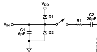
Figure 23. Equivalent Analog Input Circuit
