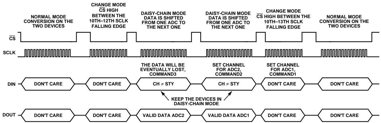
Figure 34. Daisy-Chain Diagrams—I
