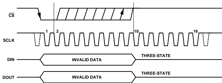
Figure 28. Entering Power-Down Mode
