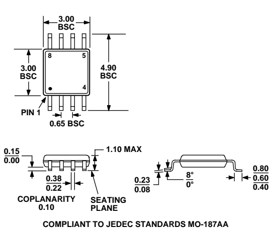
Figure 42. 8-Lead Mini Small Outline Package [MSOP] (RM-8) Dimensions shown in millimeters
