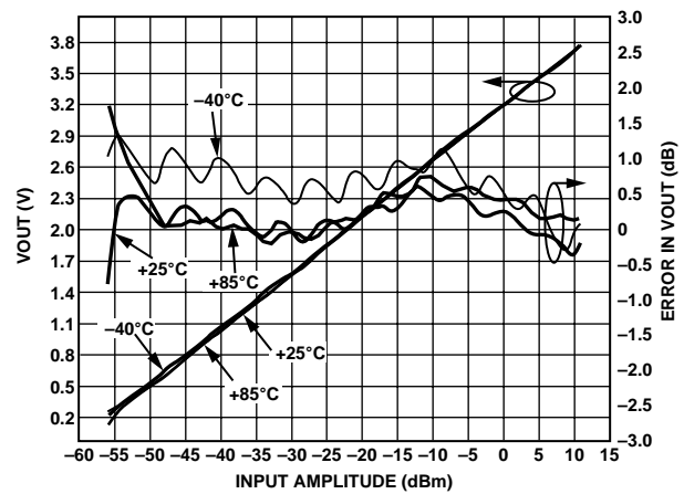
Figure 51. Output Voltage and Law Conformance Error, at T_A = -40^\circ\text{C} , +25^\circ\text{C} , and +85^\circ\text{C}
