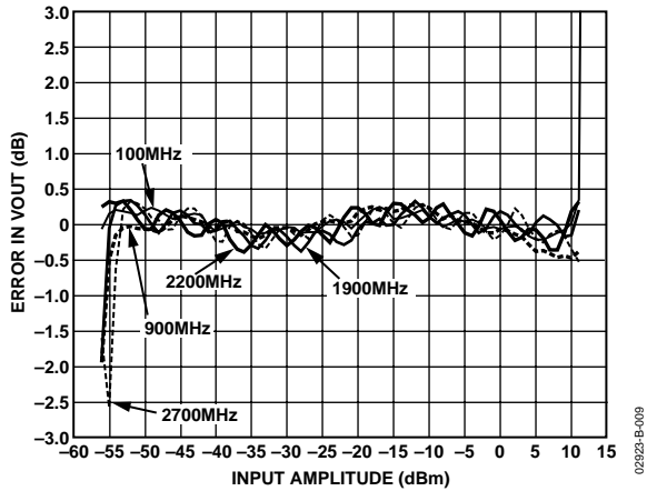
Figure 9. Logarithmic Law Conformance vs. Input Amplitude, Frequencies 100 MHz, 900 MHz, 1900 MHz, 2200 MHz, 2700 MHz, Sine Wave, Differential Drive
