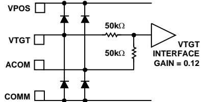
Figure 5. Circuit C
