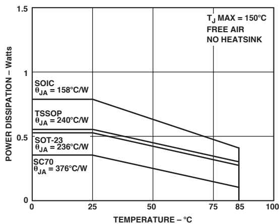
Figure 34. Maximum Power Dissipation vs. Ambient Temperature
