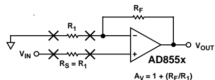
Figure 48. Mismatch in Seebeck Voltages Causes a Thermoelectric Voltage Error
