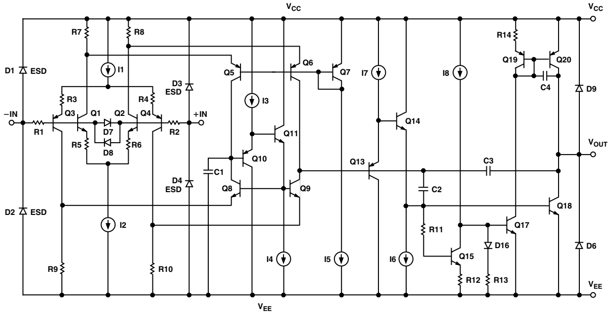
Figure 19. Simplified Schematic
