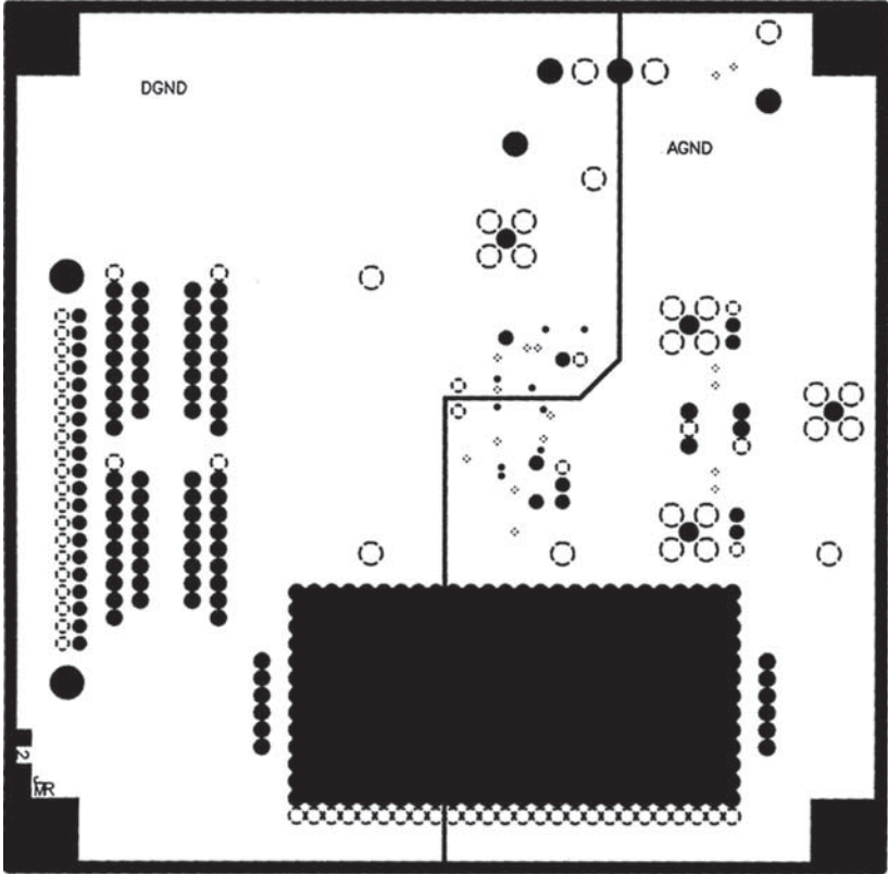
Figure 21. Ground Plane
