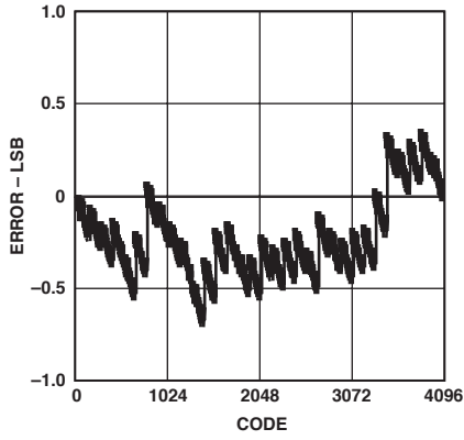
TPC 10. Typical INL
