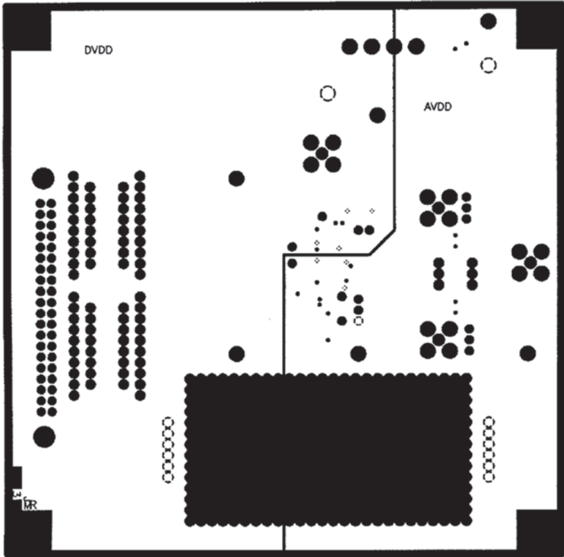
Figure 22. Power Plane
