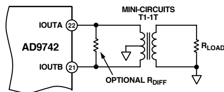
Figure 10. Differential Output Using a Transformer
