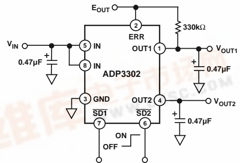
Figure 1. Application Circuit
