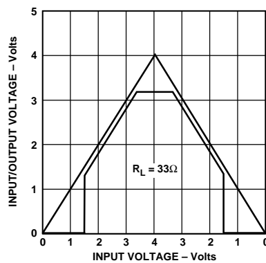
Figure 9. Power-Up/Power-Down on ADP3302AR3. S_D = 3 V or V_{IN}
