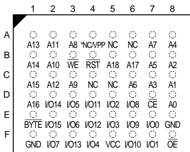
AT49BV8192A(T) CBGA Top View (Ball Down)
