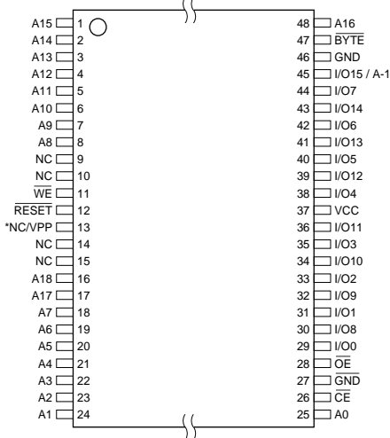
AT49BV8192A(T) TSOP Top View Type 1
