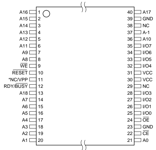
AT49BV008A(T) TSOP Top View Type 1
