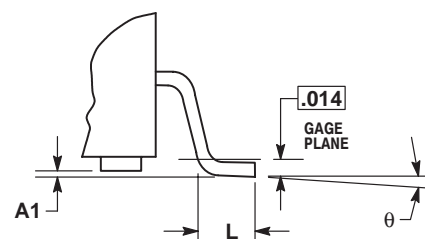
DETAIL E
