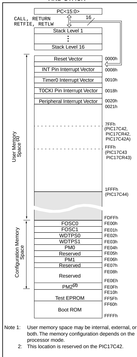
FIGURE 6-1: PROGRAM MEMORY MAP AND STACK
