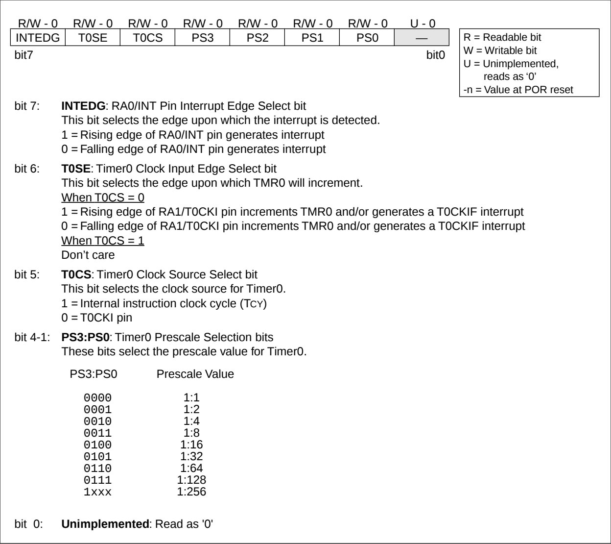
FIGURE 6-9: T0STA REGISTER (ADDRESS: 05h, UNBANKED)
