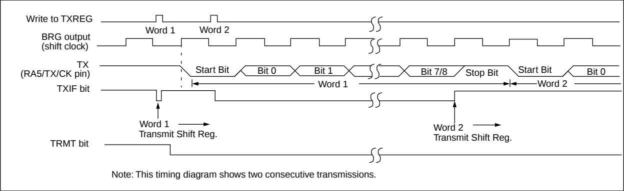
FIGURE 13-6: ASYNCHRONOUS MASTER TRANSMISSION (BACK TO BACK)
