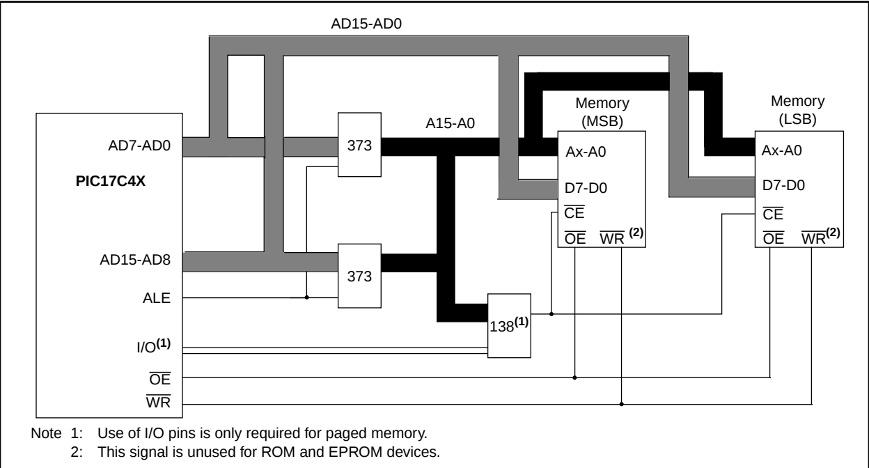
FIGURE 6-4: TYPICAL EXTERNAL PROGRAM MEMORY CONNECTION DIAGRAM
