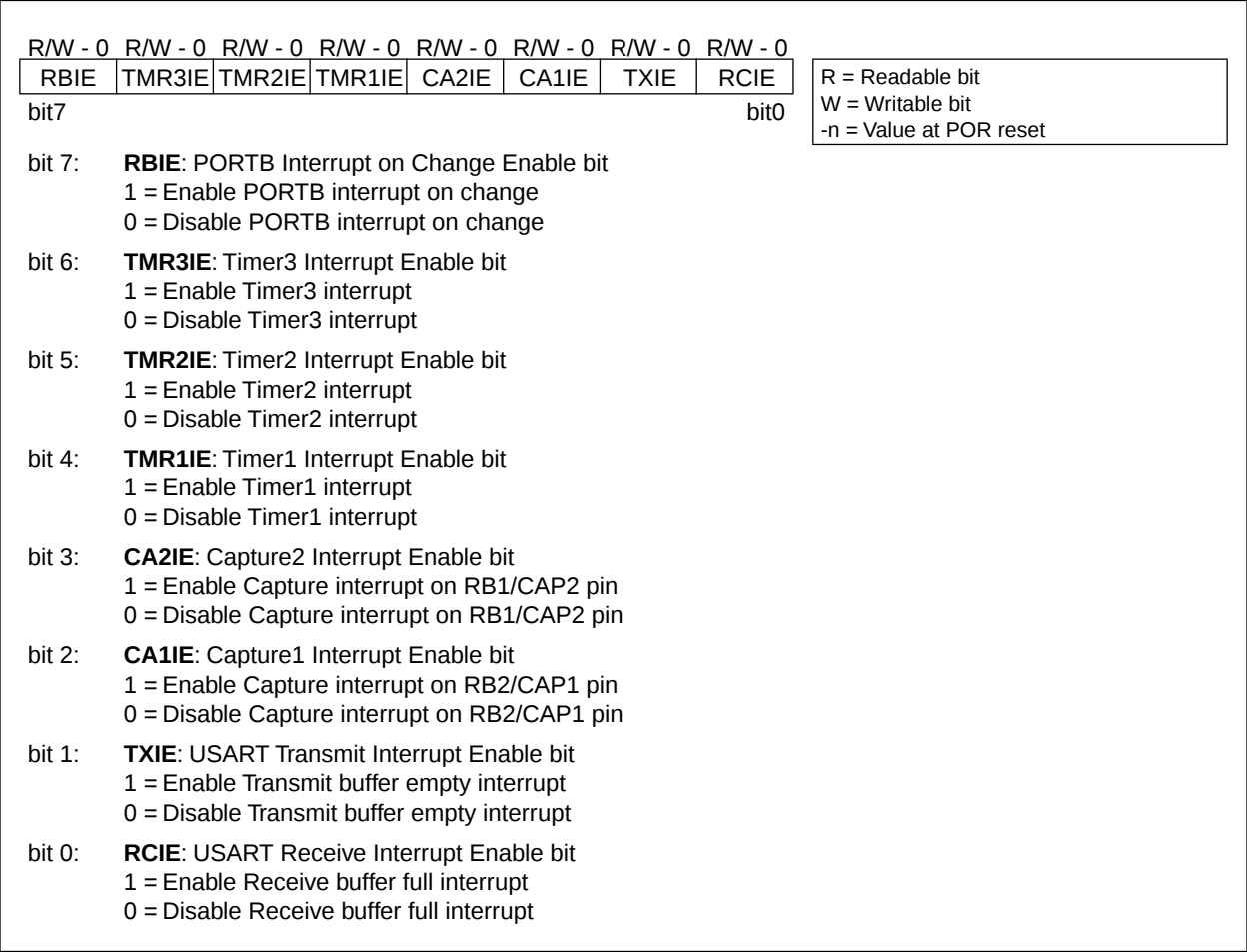
FIGURE 5-3: PIE REGISTER (ADDRESS: 17h, BANK 1)
