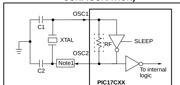
FIGURE 14-2: CRYSTAL OR CERAMIC RESONATOR OPERATION (XT OR LF OSC CONFIGURATION)
