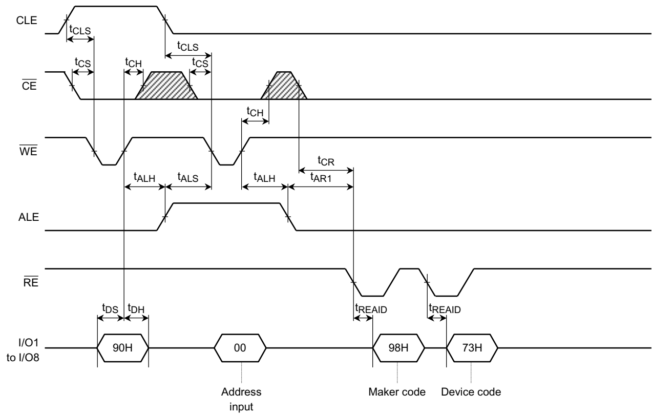
ID Read Operation Timing Diagram
