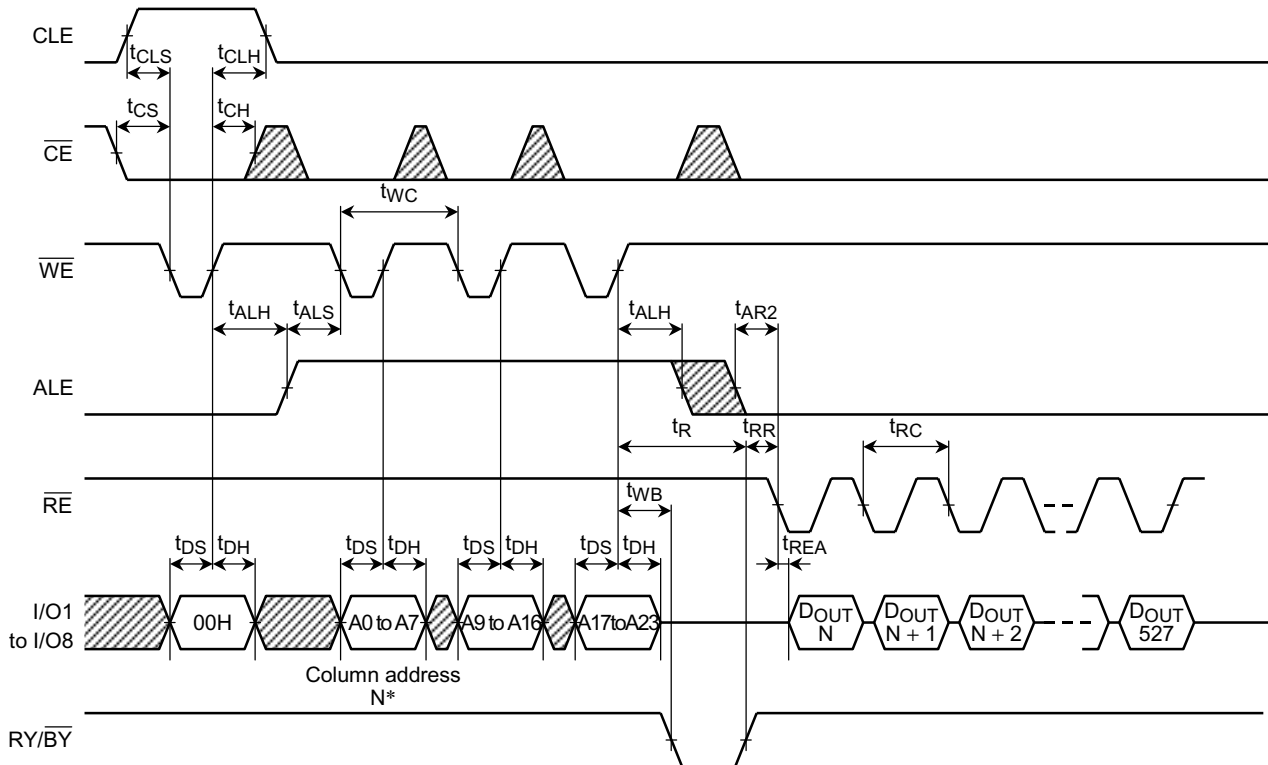
Read Cycle (1) Timing Diagram
