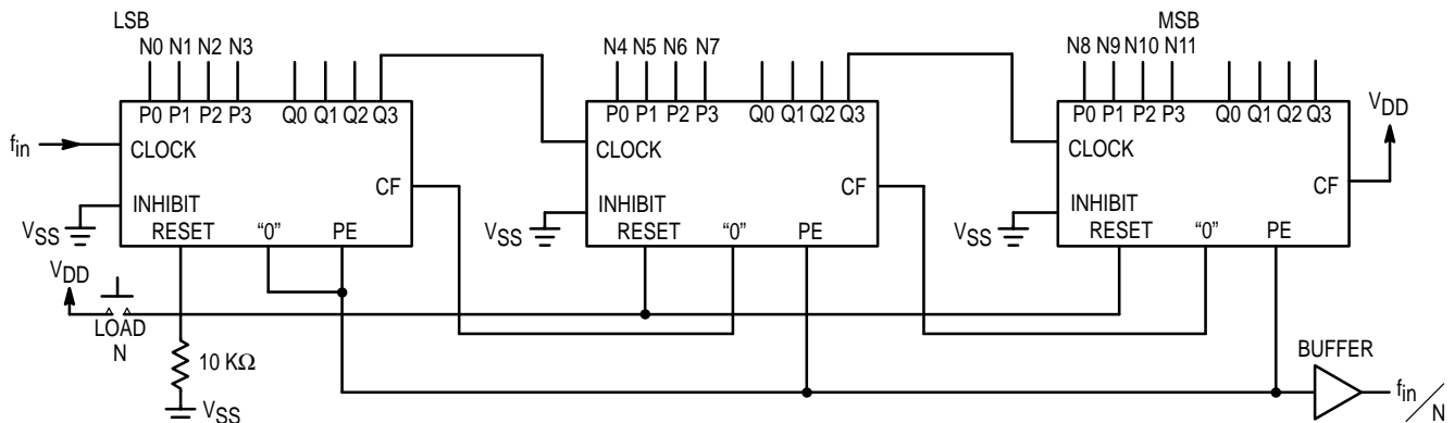
Figure 12. 3 Stages Cascaded
