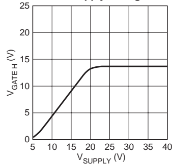
Gate to Source Voltage vs. Supply Voltage
