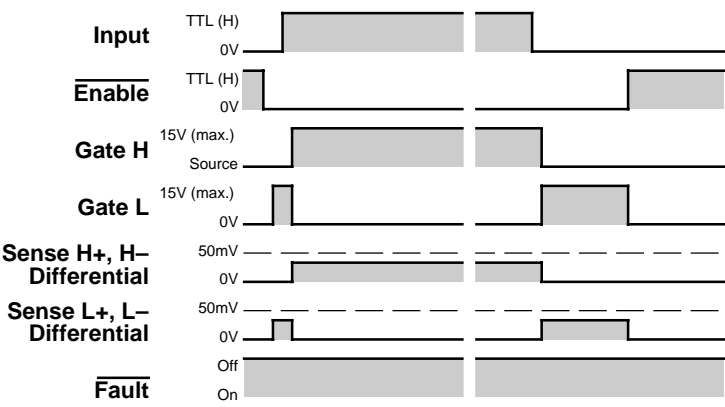
Timing Diagram 1. Normal Operation
