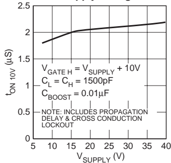
Gate Turn-On Delay vs. Supply Voltage
