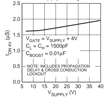
Gate Turn-On Delay vs. Supply Voltage
