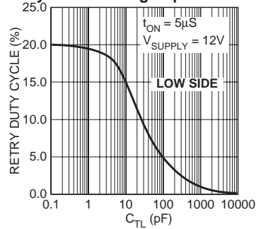
Overcurrent Retry Duty Cycle vs. Timing Capacitance
