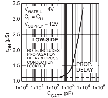
Gate Turn-On/Off Delay vs. Gate Capacitance
