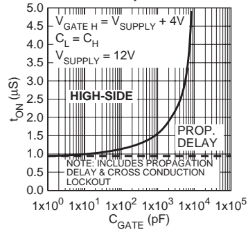
Gate Turn-On/Off Delay vs. Gate Capacitance
