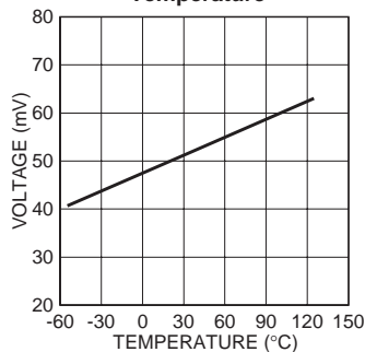
Sense Threshold vs. Temperature
