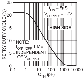
Overcurrent Retry Duty Cycle vs. Timing Capacitance
