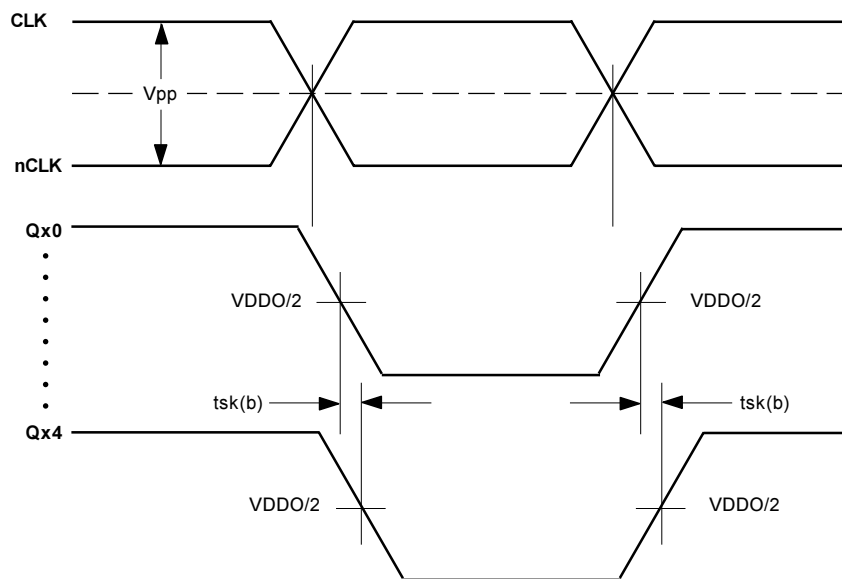
FIGURE 4A - BANK SKEW
