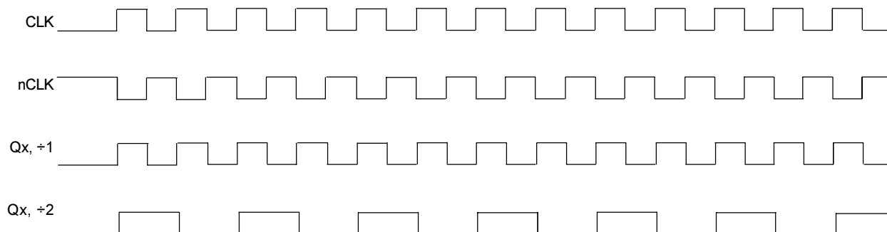
FIGURE 1A - ACTIVE, \div 1, \div 2
