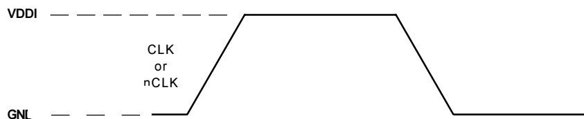
FIGURE 2C - LVCMOS AND LVTTTL SINGLE ENDED INPUT LEVEL
