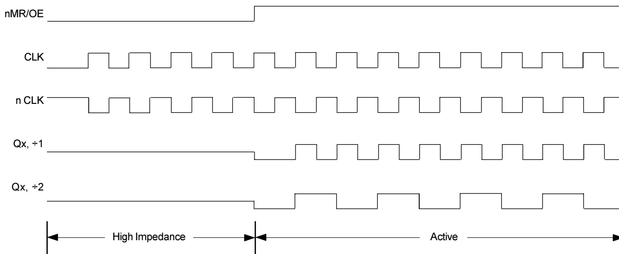
FIGURE 1B - RESET TO ACTIVE, \div 1, \div 2
