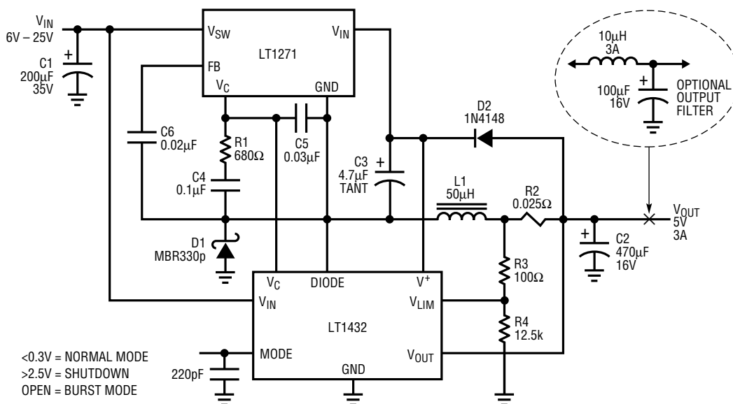
Figure 15. Adding Foldback Current Limiting
