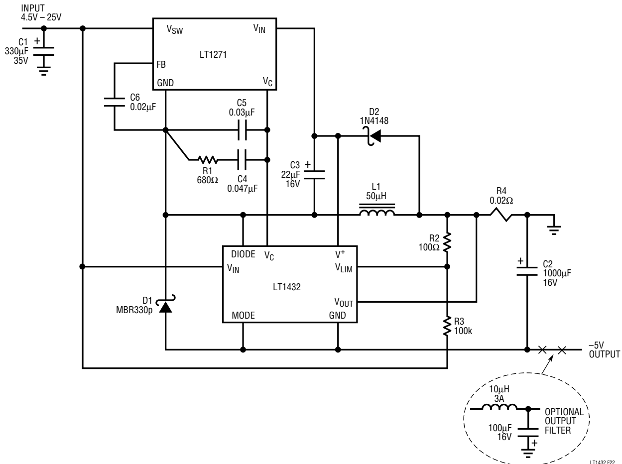
Figure 22. Positive-to-Negative Converter
