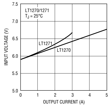
Minimum Input Voltage – Normal Mode (1270/1271)
