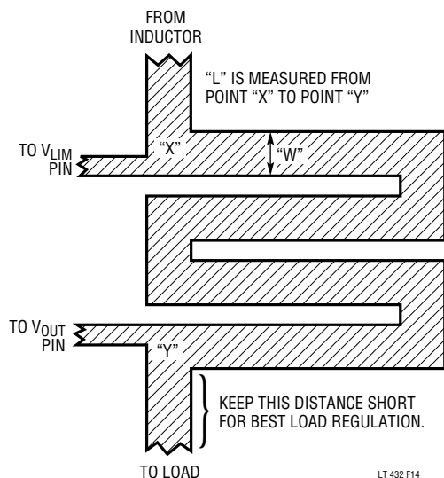
Figure 14. PC trace Current Limit Sense Resistor with Kelvin Contacts
