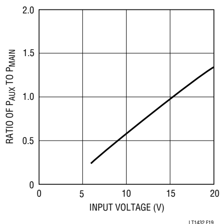
Figure 19. Auxiliary Power vs 5V Power
