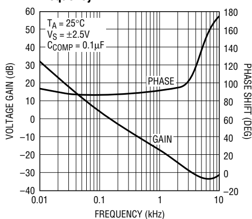
Gain and Phase Shift vs Frequency
