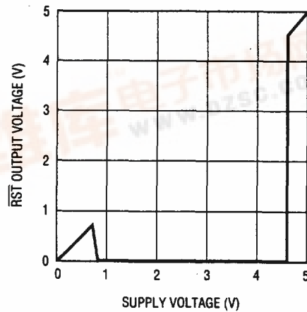
\overline{RST} Output Voltage vs Supply Voltage
