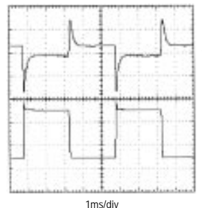
LOAD-TRANSIENT RESPONSE
