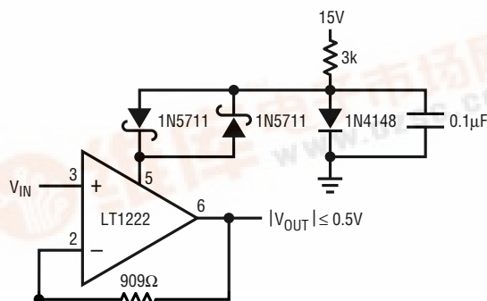
A_V = 10 with Output Clamping
