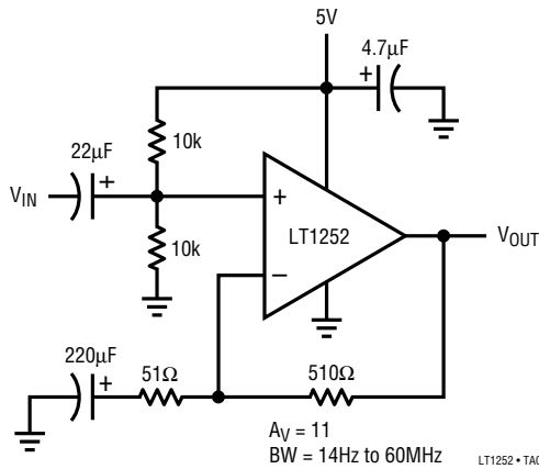
Single Supply AC-Coupled Amplifier Noninverting
