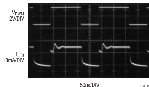
Figure 5. PWM Dimming Using the SHDN Pin
