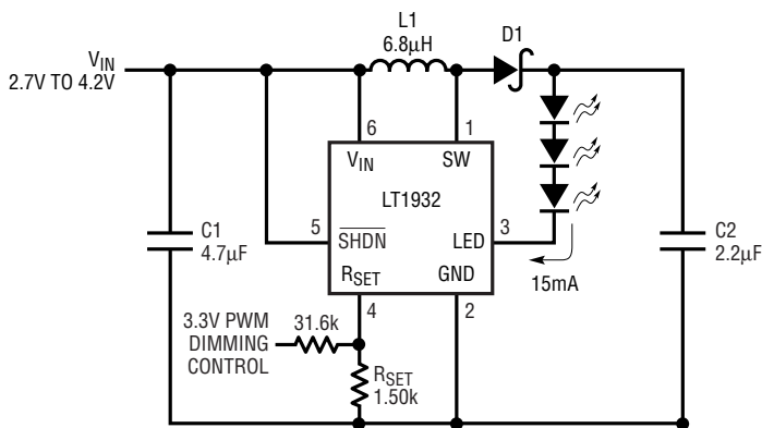
Li-Ion Driver for Three White LEDs
