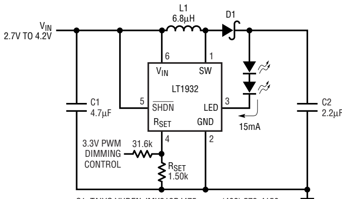
Li-Ion Driver for Two White LEDs
