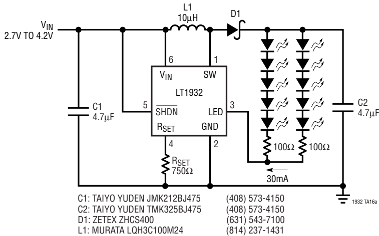
Li-Ion Driver for Ten White LEDs
