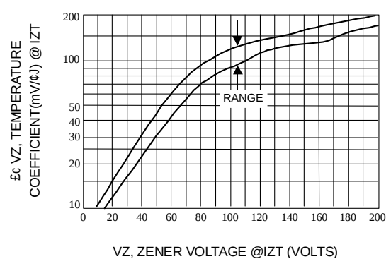
Fig. 6-UNITS 10 TO 200 VOLTS
