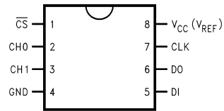
ADC08832 N,M,MM Packages
