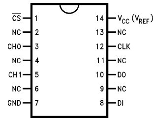
ADC08832 Wide Body SO Packages
