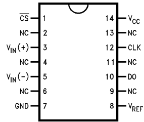
ADC08831 Wide Body SO Packages
