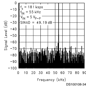
Spectral Response with 55 KHz Sine Wave Input
