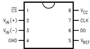
ADC08831 N,M,MM Packages
