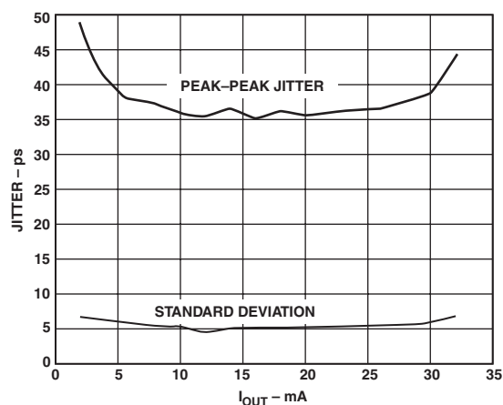
TPC 18. Jitter vs. Programmed I_{OUT}
