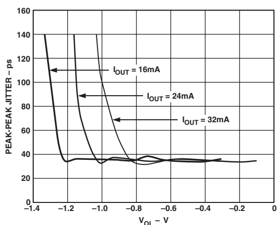
TPC 17. Jitter vs. V_{OL} (Relative to VCC)
