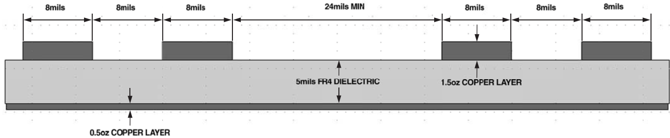
Figure 12. Cross-Sectional Layout and Dimensioning (To Scale) of Differential
