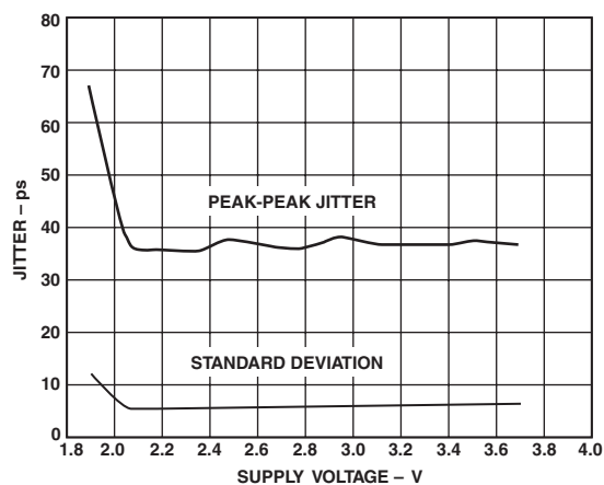
TPC 16. Jitter vs. Supply
