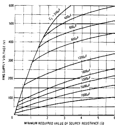
Fig. 3 - Minimum Required Source Resistance Vs. RMS Supply Voltage and Load Capacitance
