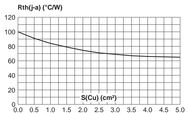
Fig. 8: Thermal resistance junction to ambient versus copper surface under each lead (Epoxy printed circuit board FR4, copper thickness: 35µm).
