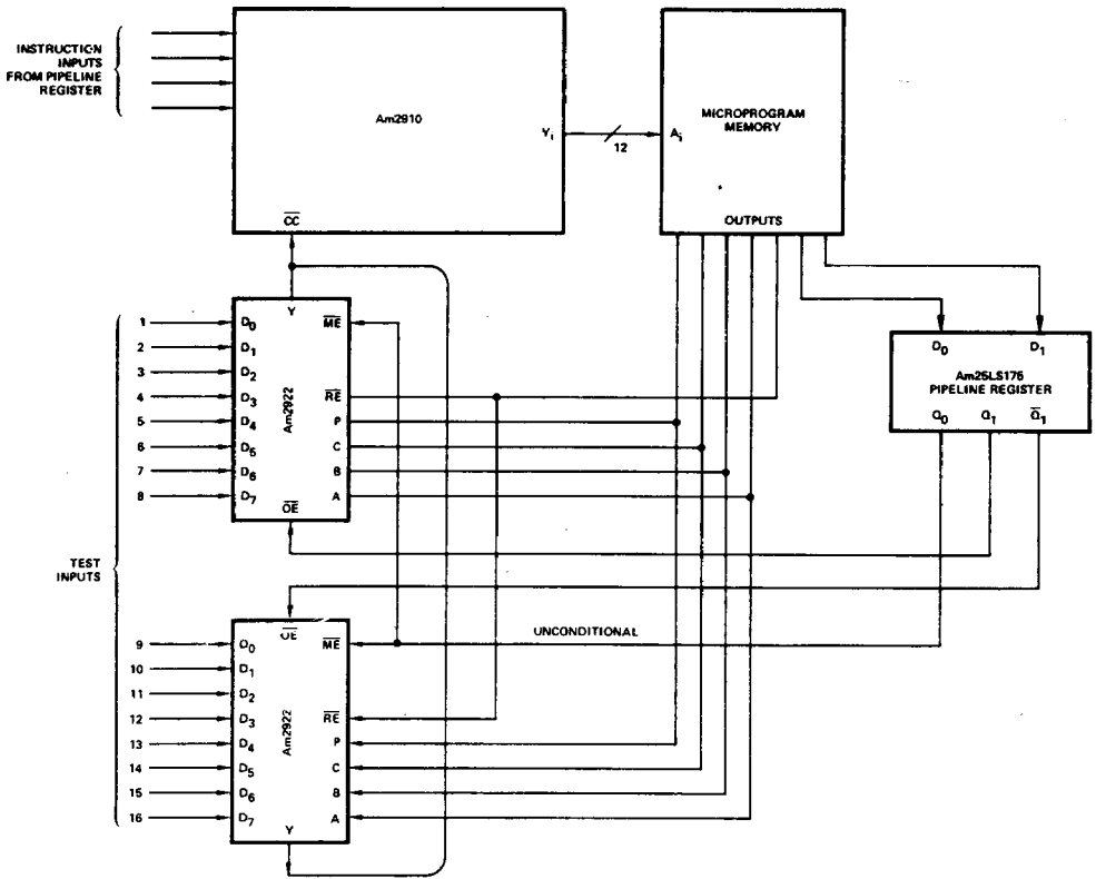
A versatile one-of-sixteen Test Select with Polarity Control and Test Select Hold.
