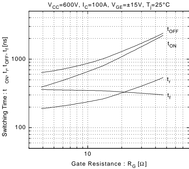
Switching Time vs. R_G
