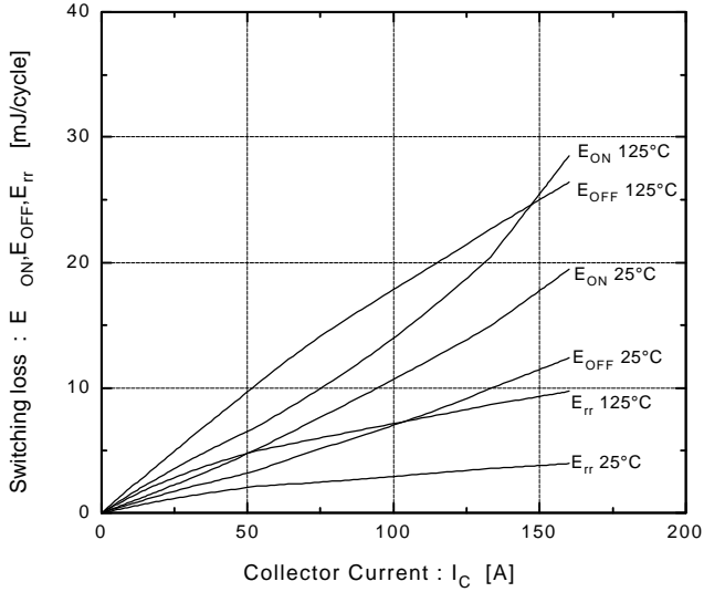
Switching loss vs. Collector current V_{CC}=600V, R_G=9.1\Omega, V_{GE}=\pm 15V
