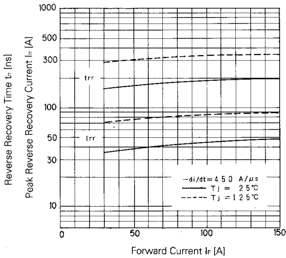
T_{rr}, I_{rr}-I_f
