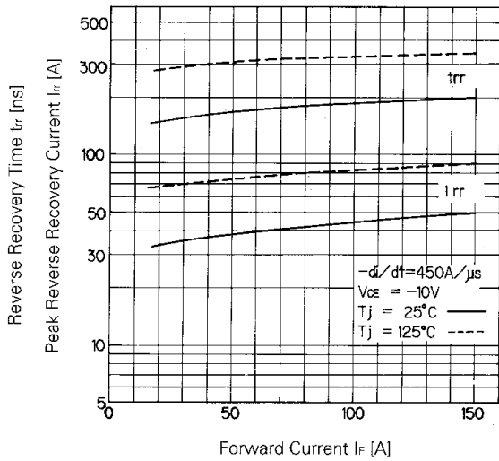
t_{rr}, I_{rr}-I_f
