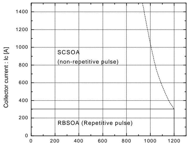
Reversed biased safe operating area +V_{GE}=15V, -V_{GE}\le 15V, T_J\le 125^\circ C, R_G\ge 5.6\Omega
