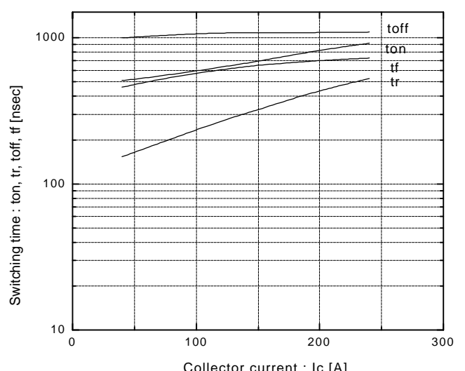
Switching time vs. Collector current V cc =600V, R G =5.6Ω, V GE =±15V, T j =125°C
