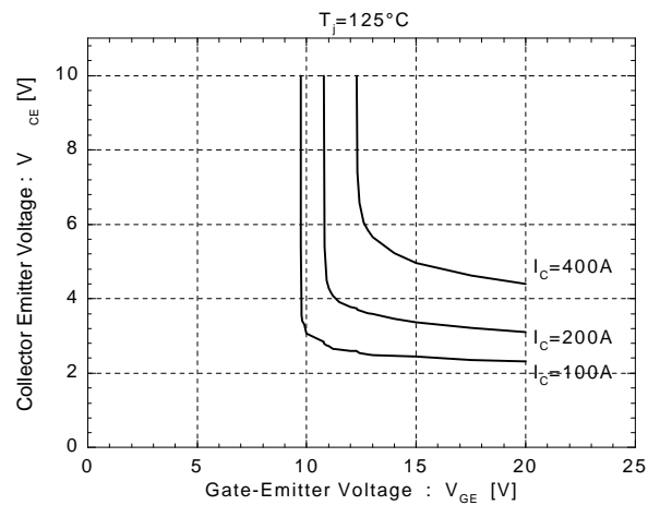
Collector-Emitter vs. Gate-Emitter Voltage
