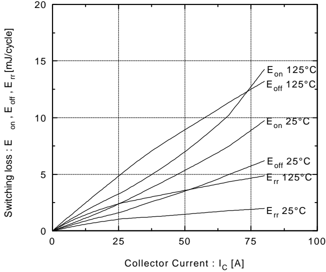
Switching loss vs. Collector current V_{CC}=600V, R_G=24\Omega, V_{GE}=\pm 15V
