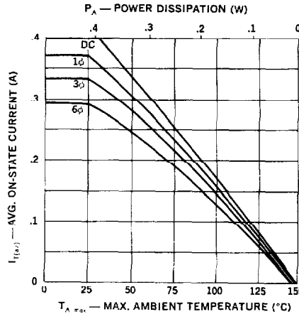
C6 Average Current vs. Ambient Temperature TO-18 Ratings (see note) P_A — POWER DISSIPATION (W)
