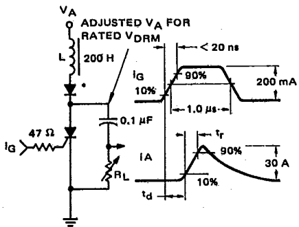
FIGURE 1 - TURN-ON TIME
