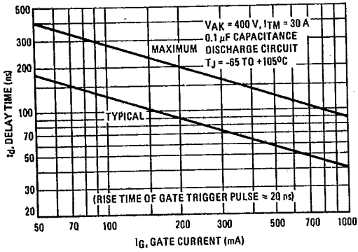
FIGURE 9 - DELAY TIME
