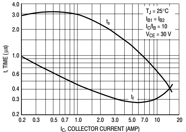
Figure 6. Turn-Off Time
