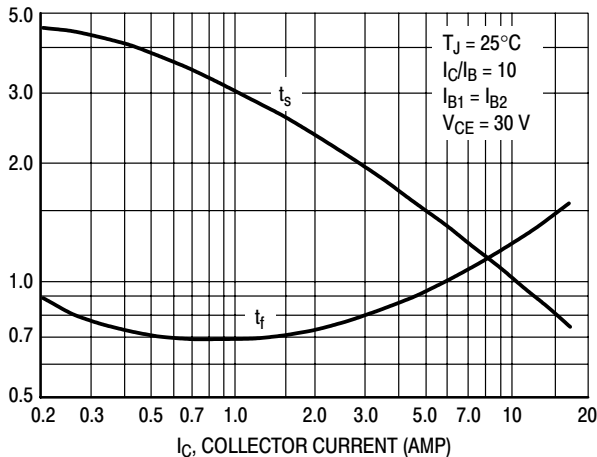
Figure 6. Turn-Off Time
