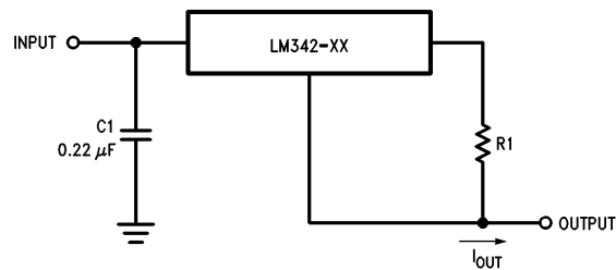
Current Regulator
